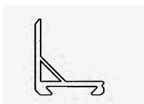
Side Mount Plate *SOLD SEPARATELY
