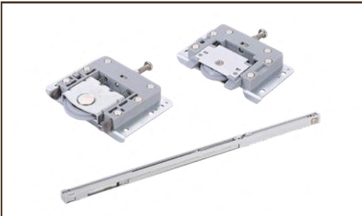
4pcs Upper Runner, 4pcs Down Runner and 4pcs Damper
